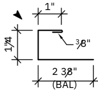
COMMERCIAL "J" TRIM (5" GIRTH)
