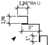
COMMERCIAL INSIDE CORNER (14" GIRTH)
