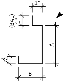
SLIDING DOOR EDGE TRIM (A + B + 3/4" GIRTH)
