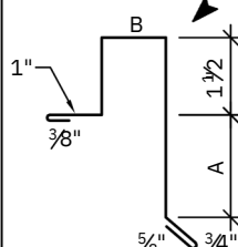
GABLE END CAP FOR "HERITAGE" PROFILE (A+B+5 3/4" = GIRTH)
