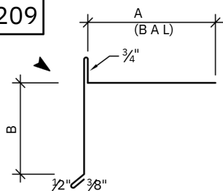
GRAVEL STOP (A + B + 3/8" = GIRTH)
