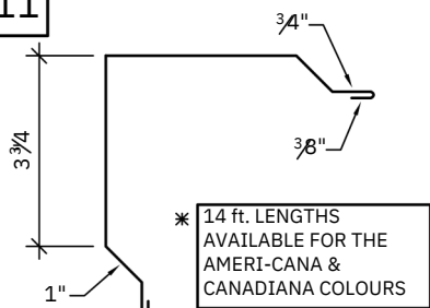
RAKE EDGE TRIM (12" GIRTH) (10 or 14 ft. LENGTHS) *
