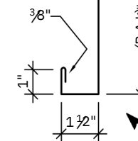
FASCIA: TYPE 1 (9" GIRTH)
