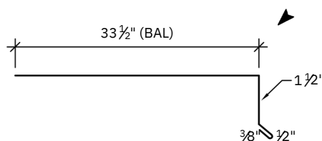
ICE APRON (for shingles) (36" GIRTH)
