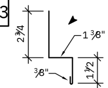
GABLE DIVIDER (6" GIRTH)
