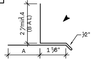
INDUSTRIAL WINDOW & DOOR FLASHING (A + 7" = GIRTH)
