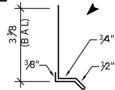
COLONIAL WINDOW & DOOR FLASHING (6" GIRTH)
