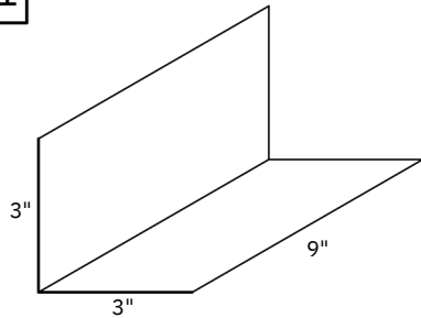
STEP FLASHING (6" X 9") (50 PCS PER BUNDLE) (MIXED COLOURS)
