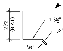
INDUSTRIAL BASE FLASHING (5" GIRTH)
