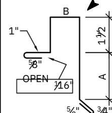
GABLE END CAP FOR "HERITAGE" PROFILE (A+B+6" = GIRTH)
