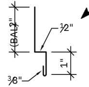
COLONIAL GABLE DIVIDER (4" GIRTH)
