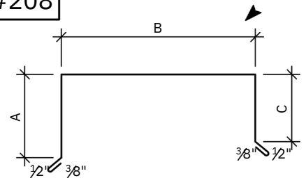
CAP FLASHING (A + B + C + 3/4" = GIRTH)
