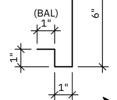
FASCIA: TYPE 2 (9" GIRTH)
