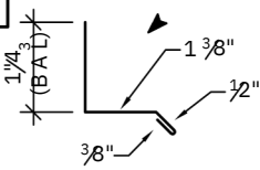
COMMERCIAL BASE FLASHING (4" GIRTH)
