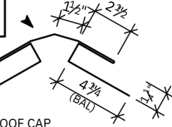
COTTAGE ROOF CAP FOR COMMERCIAL RIB PROFILE (24" GIRTH)
