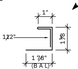
INDUSTRIAL "J" TRIM (7" GIRTH)
