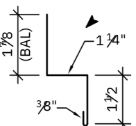
COMMERCIAL GABLE DIVIDER (5" GIRTH)
