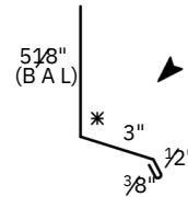
WALL FLASHING TYPE S (9" GIRTH) * SPECIFY PITCH
