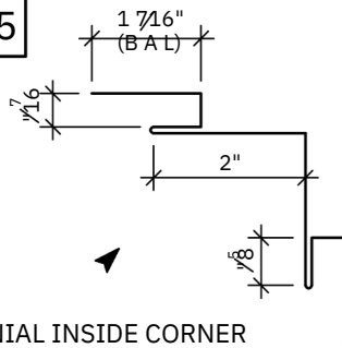
COLONIAL INSIDE CORNER (9" GIRTH)
