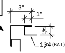
COMMERCIAL OUTSIDE CORNER (14" GIRTH)
