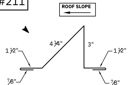
SNOW GUARD (12" GIRTH) MINIMUM 26g (.021") RECOMMENDED
