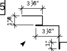
INSIDE CORNER (18" GIRTH)
