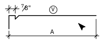
SINGLE SOFFIT: TYPE 1J (A+3" = GIRTH)
