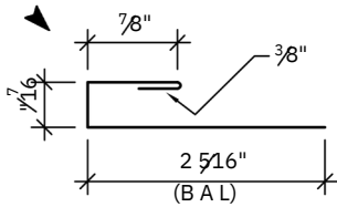
COLONIAL "J" TRIM (4" GIRTH)
