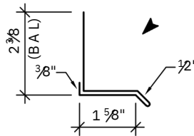
INDUSTRIAL WINDOW & DOOR FLASHING (7" GIRTH)
