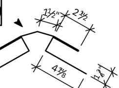
COTTAGE ROOF CAP (24" GIRTH)
